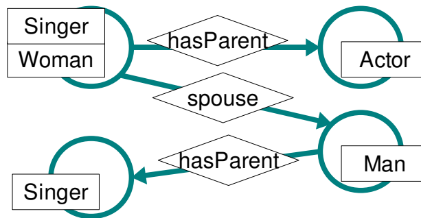
Illustration 8: Query Tool query for \text{Singer} \sqcap \text{Woman} \sqcap \exists \text{hasParent} . (\text{Actor}) \sqcap \exists \text{spouse} . (\text{Man} \sqcap \exists \text{hasParent} . (\text{Singer}))
