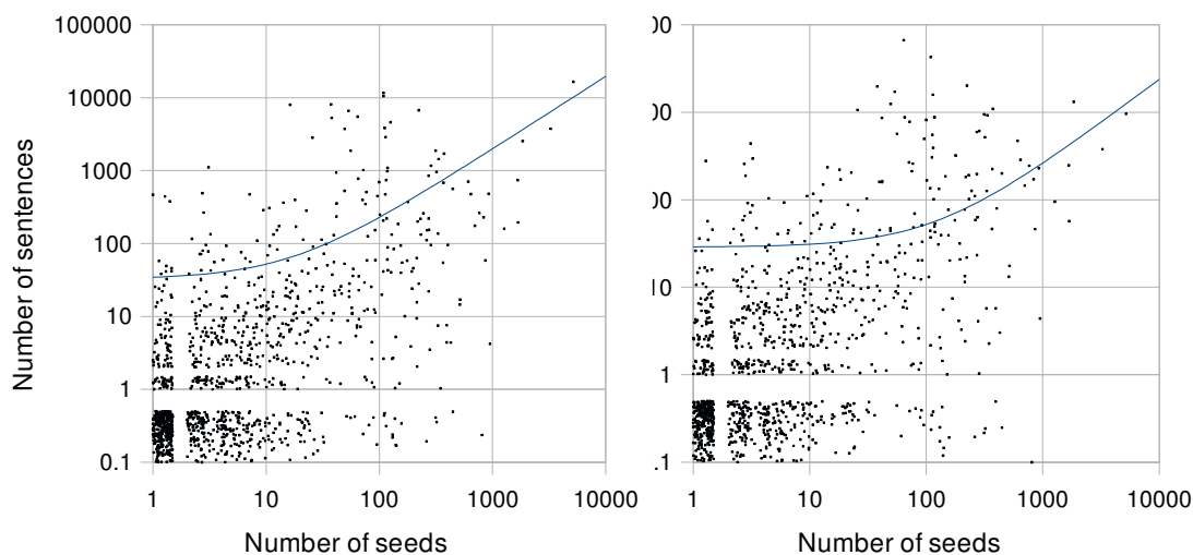
Illustration 15: Relations scattered on the real plane according to the number of their seeds and the number of their sentences and paths
